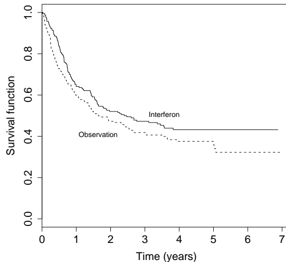
Figure 6: Kaplan-Meier curves of high-dose interferon and observation groups in cutaneous melanoma data.
