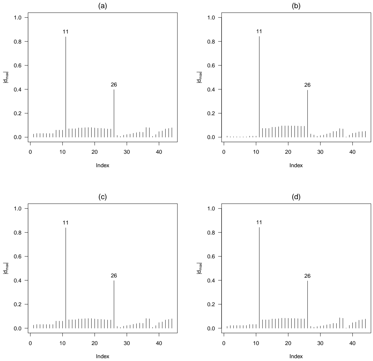
Figure 5: Influence index plots (case weight perturbation) for the L\beta BS (a), LEBS (b), LLeBS (c) and LBS (d) models.
