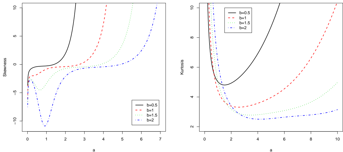
Figure 2: Skewness and kurtosis of Y in (4) as a function of a for some values of b .
