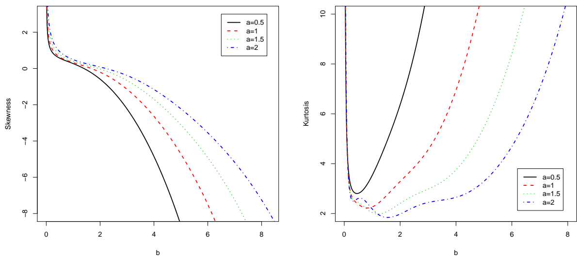
Figure 3: Skewness and kurtosis of Y in (4) as a function of b for some values of a .
