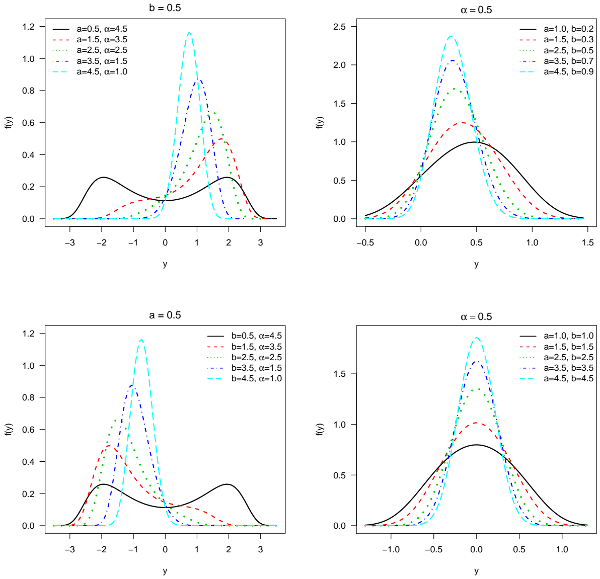
Figure 1: Plots of the density function (4) for some parameter values: \mu = 0 and \sigma = 1 .
