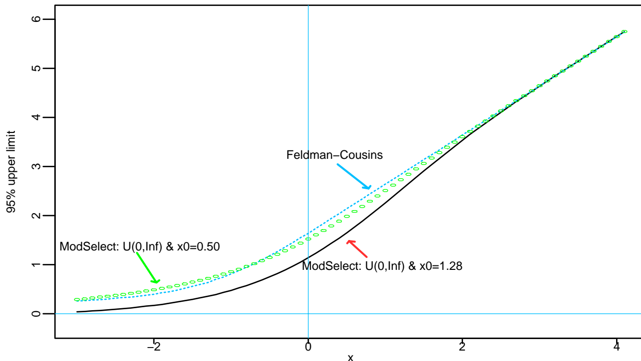
Figure 4: Moving the break-even point x_0 , (17), closer to zero makes the Model Selection upper 95% point nearly match the Feldman-Cousins bound.
