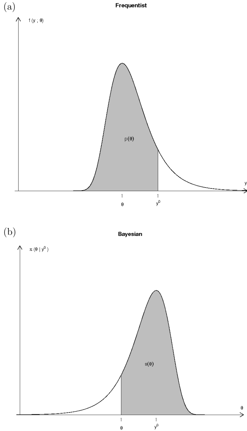
Figure 2: The extreme value EV(\theta,1) model: the density of y given \theta in (a); the posterior density of \theta given y^0 in (b): the p -value p(\theta) from (a) is equal to the survivor value s(\theta) in (b).
