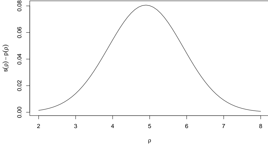
Figure 8: The Bayes error s(\rho) - p(\rho) with data r^0 from the N(\theta, I) model with data y^0 = (5, 0) .
