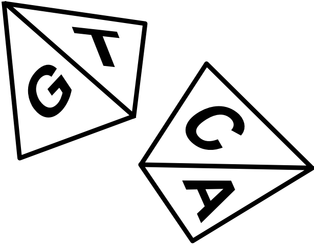
Figure 1: DNA dice.
