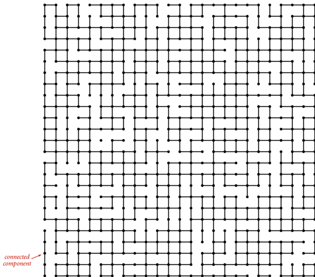
Medium connectivity example (625 sites, 900 edges, 3 connected components)
